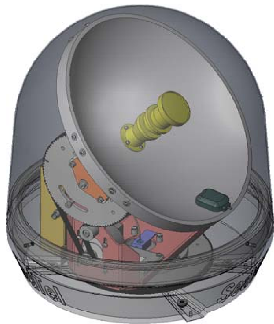
Coastal 14M TVRO Antenna (with Ku-Band LNB)
