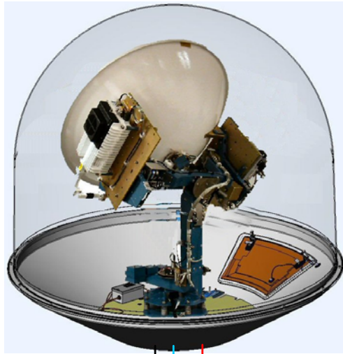
4006RZA Above Decks Equipment
