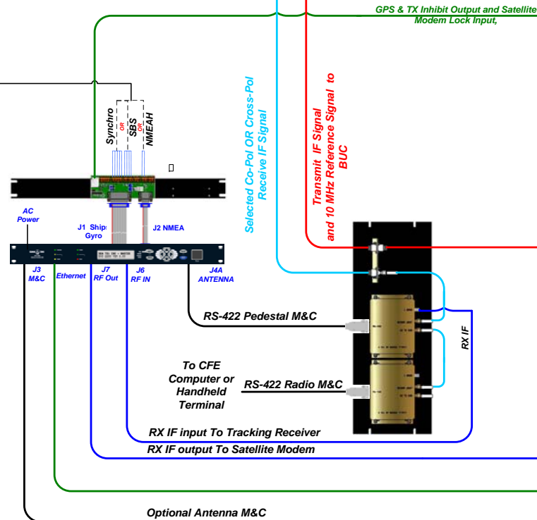
Terminal Mounting Strip
