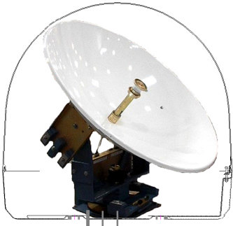
Coastal Series Antenna with US or DLA LNB Antenna "A"
