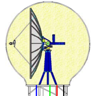
Series 97B/00B-21 Dual C/Quad Ku Linear Feed Antenna "B"
