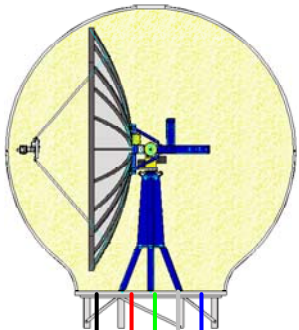
Series 97B/00B-21 Dual C/Quad Ku Linear Feed Antenna "A"
